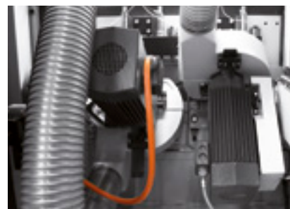
Swivel-mounted high-frequency motors with individual extraction system
