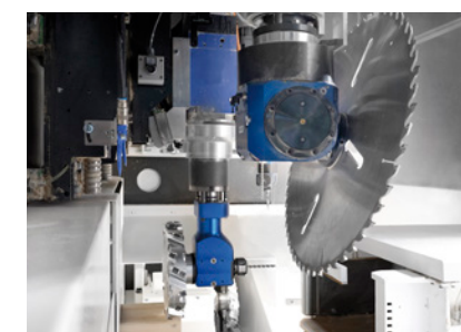
Second integrated main spindle
