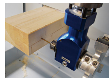
Horizontal drilling
