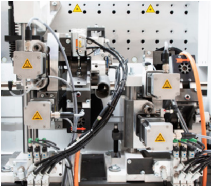
BF40/MS40 trimming unit
