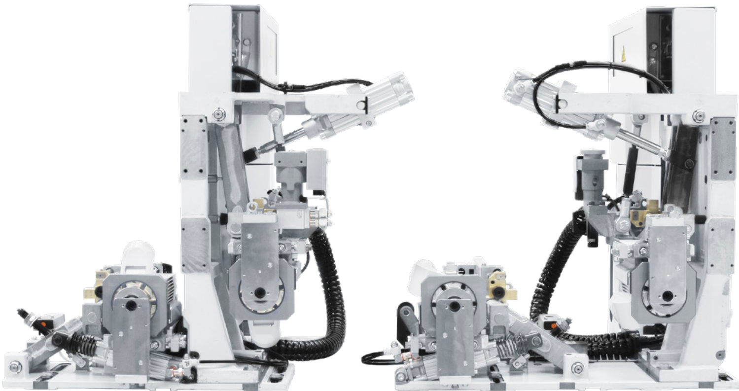
FF32 profile trimming unit
