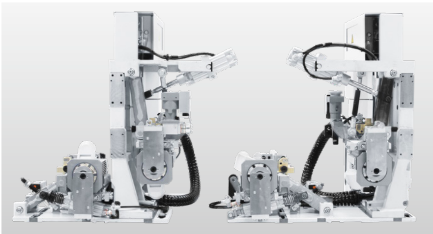
FF32 profile trimming unit
