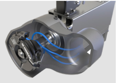
Controlled chip collection The chips are suctioned off in the interior and fed to the extraction hood in a targeted manner. Reduced wear and tear and lower service costs increase profitability and service life. The reduced suction speed lowers energy consumption and costs.
