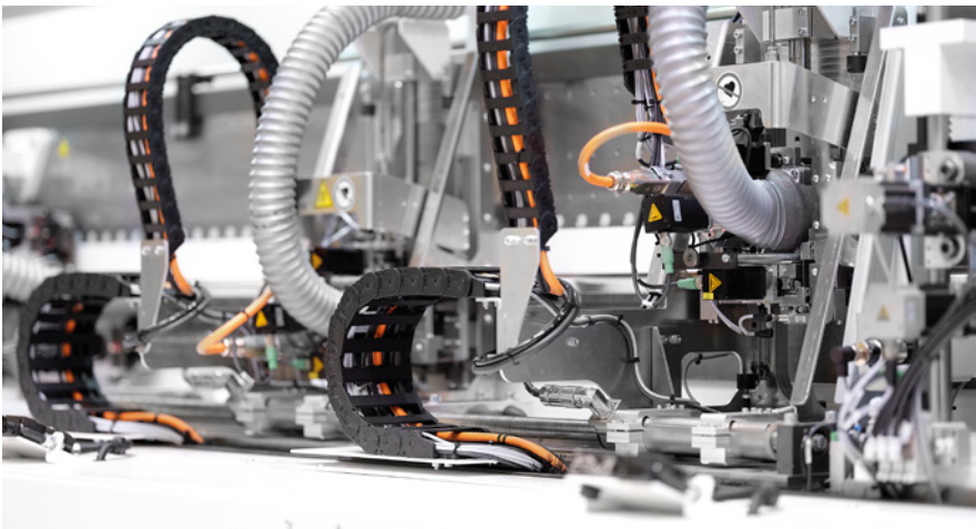
MF60 Servotrim multifunction profile trimming unit
