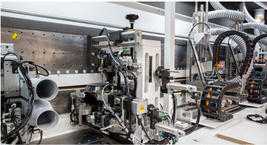
MN11 multi-scraper
