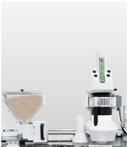
Combination of melting units for optional processing of EVA and PUR
