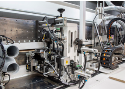
MN11 profile scraper
