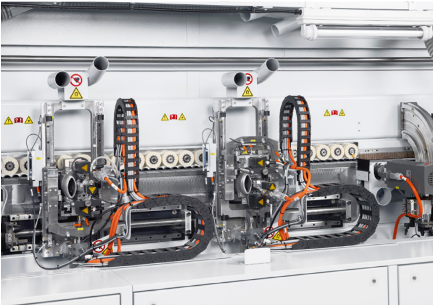
MF60 Servotrim multifunction profile trimming unit For processing edge overhangs on the upper and bottom edge of the workpiece and for corner rounding of the front and rear edge. Servo-controlled motion sequence with Soft Touch function, for optimum processing of high-gloss surfaces or lightweight panels, for example. Workpiece thickness 60 mm.
