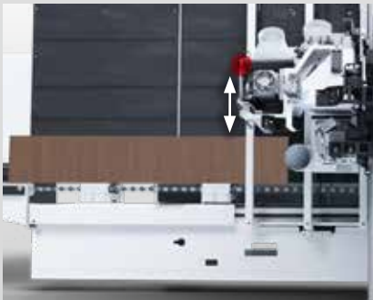
▪ Determination of the exact workpiece length (value 2).
