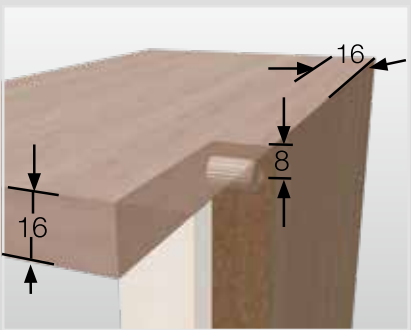
▪ Dimension-dependent holes are automatically corrected by any tolerances determined.
