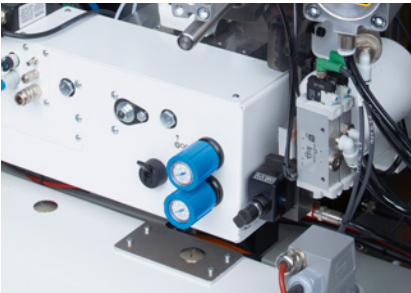
Magazine height adjustment: The edge overhang on the underside can be increased by adjusting the magazine plate. (Optional for 1120 F and 1130 FC models)
