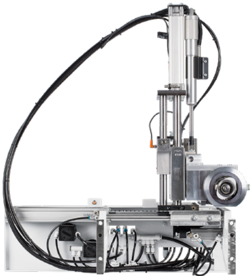
FF6210 profile trimming unit Optimum profile trimming without making adjustments thanks to the linked DIA tool and detector roller. With an optional automatic adjustment between thin and thick edges.
