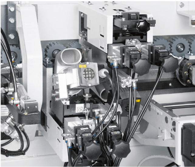
Trimming unit with pneumatic three-point adjustment (optional) For more efficient production and significant time savings during changeover.
