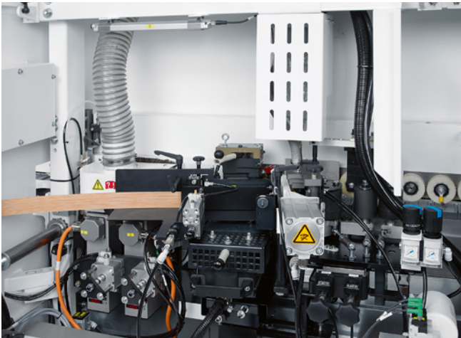
Easy integration The airTec reactivation unit is installed in such a way that you can work with either the standard application unit or the airTec system. Image of EDGETEQ S-200 model 1110 AT, 1120 AT and 1130 AT.
