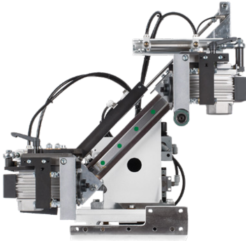
Snipping unit Exact snipping cut via a robust snipping unit with a highly precise linear guide. Automatic chamfer/straight adjustment included as standard on the 1130 FC, 1120 F and 1130 AT models.
