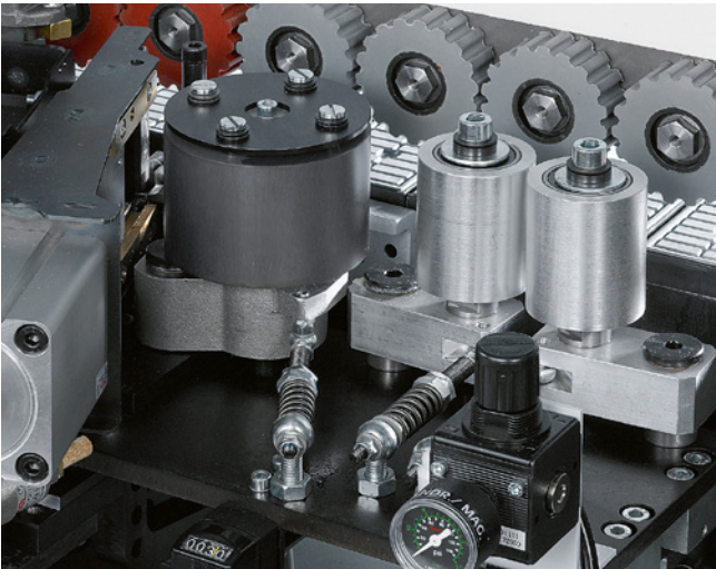
EDGETEQ S-200 pressure zone Pressure zone up to an edge thickness of 3 mm and a panel height of 40 mm for optimum glue joint quality.
