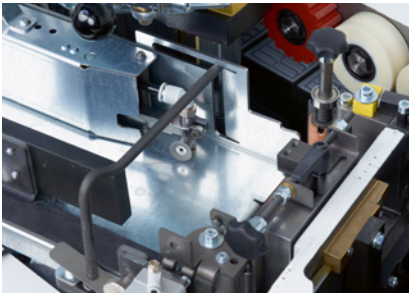
Strip separation: The use of a vacuum suction unit makes it very easy to separate thin veneer, HPL or composite strips with an edge thickness of 0.4 to 1.0 mm. (Optional for 1120 F, 1130 FC and 1130 AT models)
