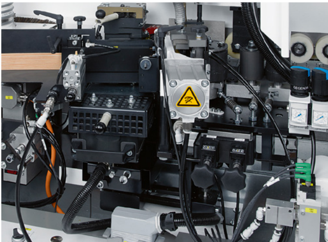
Gluing stations Quick-change application unit with hot-melt glue supply from below. Can process PUR granulate.
