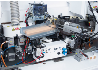
Servo edge feed: The direct drive enables a more precise edge position without gears and drive units, which increases the durability and operational safety and reduces the maintenance effort. (Standard on 1120 F, 1130 FC and 1130 AT models)
