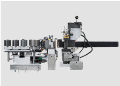
Gluing stations for safe hot-melt glue application HOMAG gluing stations are ideal for quick, solid gluing. The heated gluing roller ensures an optimal glue temperature.
